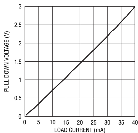
\overline{\text{INT}} and SDAOUT Pull Down Voltage vs Load Current
